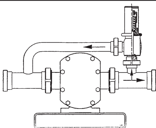
EXTERNAL PRESSURE RELIEF VALVE
