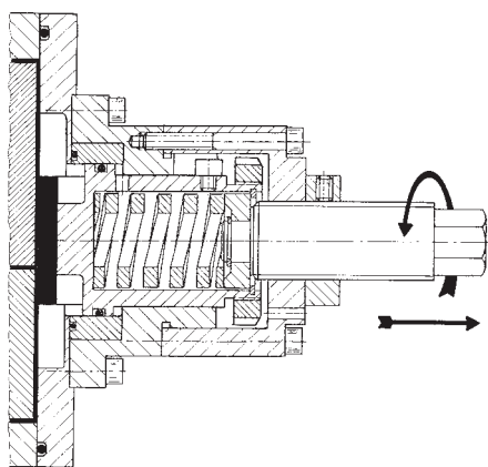
INTEGRAL PRESSURE RELIEF VALVE
